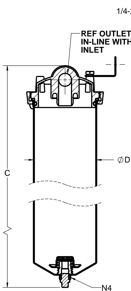
SECTION B-B
