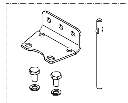
ITEMS 8 & 9 MOUNTING BRACKET (hardware included) & TOOL, CLAMP RING
