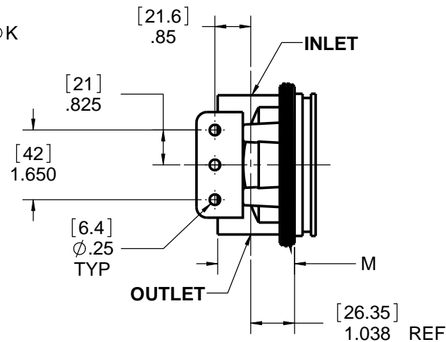
SIDE VIEW OF HEAD & BRACKET, ITEMS 2 & 8, ONLY.
