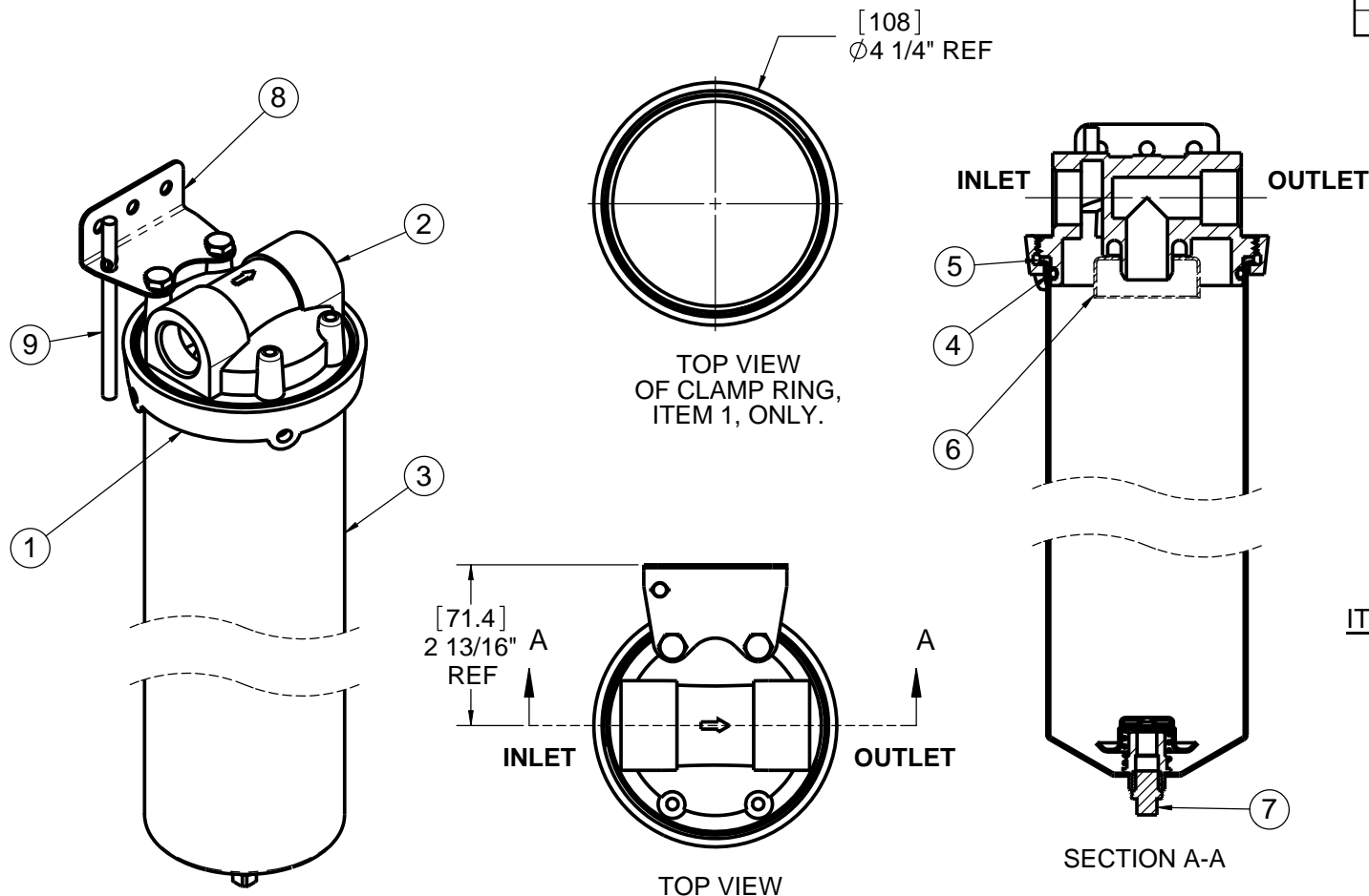
ISOMETRIC VIEW
